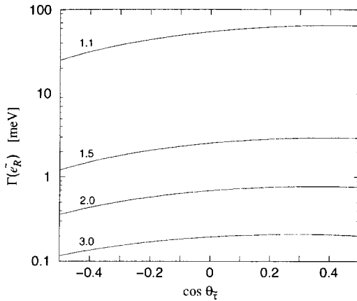
Fig. 4. The dependence of \Gamma(\tilde{e}_R \rightarrow e\tau\tilde{\tau}_1) (including both charge final states) on \cos \theta_{\tilde{\tau}} , computed as in Fig. 2 but with \Delta m = m_{\tilde{e}_R} - m_{\tilde{\tau}} - m_{\tau} held fixed at 1.0 GeV. The four curves correspond to r_{\tilde{N}_1} = 1.1, 1.5, 2.0, and 3.0 (from top to bottom).
