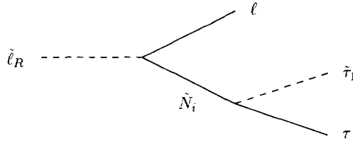
Fig. 1. Right-handed selectrons and smuons can decay according to \tilde{\ell}_R^- \rightarrow \ell^- \tau^+ \tilde{\tau}_1^- or \tilde{\ell}_R^- \rightarrow \ell^- \tau^- \tilde{\tau}_1^+ , with different matrix elements, through virtual neutralinos \tilde{N}_i ( i = 1, 2, 3, 4 ).
