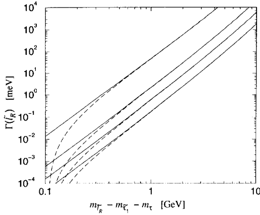
Fig. 2. The decay widths in meV for \bar{\ell}_R \rightarrow e\tau\bar{\tau}_1 (solid lines) and \bar{\mu}_R \rightarrow \mu\tau\bar{\tau}_1 (dashed lines), including both \tau^+\bar{\tau}_1^- and \tau^-\bar{\tau}_1^+ final states, as functions of \Delta m = m_{\bar{\ell}_R} - m_{\bar{\tau}_1} - m_\tau . The widths have been computed using Eqs. (21)–(26) with m_{\bar{\ell}_R} = 90 GeV, \cos\theta_{\bar{\tau}} = -0.15 and r_{\bar{N}_1} = 1.1, 1.5, 2.0, and 3.0 (from top to bottom), with the approximation N_{11} = 1 and N_{12} = N_{13} = 0 .
