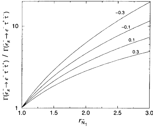
Fig. 3. The ratio \Gamma(\tilde{e}_R^- \rightarrow e^- \tau^- \tilde{\tau}_1^+) / \Gamma(\tilde{e}_R^- \rightarrow e^- \tau^+ \tilde{\tau}_1^-) is shown as a function of r_{\tilde{N}_1} , for four values of \cos \theta_{\tilde{\tau}} = -0.3, -0.1, 0.1 and 0.3 (from top to bottom). The widths have been computed using Eqs. (21)–(26) with m_{\tilde{e}_R} = 90 GeV, and with the approximation N_{11} = 1 and N_{12} = N_{13} = 0 .
