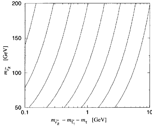
Fig. 5. Contours of constant total decay width \Gamma(\tilde{e}_R \rightarrow e\tau\tilde{\tau}_1) (from left to right, 0.0001, 0.001, 0.01, 0.1, 1, 10, 100 and 1000 meV), including both charge channels for the final state, and computed with r_{\tilde{N}_1} = 1.5 and \cos\theta_{\tilde{\tau}} = -0.15 with the same approximations as in Figs. 2–4.
