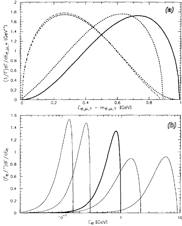
Fig. 6. Lepton energy distributions in the rest frame of the \tilde{\ell}_R^- decaying to \ell^- \tau^- \tilde{\tau}_1^+ . (a) Normalized distributions for both the final \ell (solid and dashed lines) and \tau (circles and dot-dashed line) for an ideal model with N_{11} = 1 ; N_{12} = N_{13} = 0 ; m_{\tilde{\ell}_R} = 90 GeV; \Delta m = m_{\tilde{\ell}_R} - m_{\tilde{\tau}_1} - m_\tau = 1 GeV; \cos \theta_{\tilde{\tau}} = -0.15 and r_{\tilde{N}_1} = 1.1 . Distributions for the other charge channel are almost identical. The solid line and the circles (dashed and dot-dashed lines) refer to the case \ell = e ( \ell = \mu ). (b) The logarithmic version of the solid thick curve in (a) compared to normalized electron-energy distributions in four GMSB models chosen from Ref. [9] (thin lines). \Delta m is 0.16, 0.30, 2.2, 9.7 GeV respectively from left to right, other details can be found in the text.
